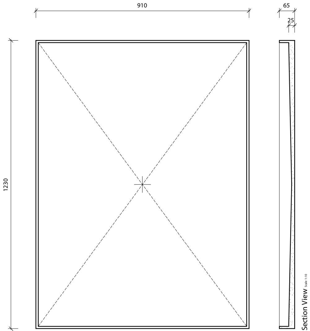
Plan View Scale 1:10
