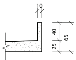
Lip Detail Scale 1:5
