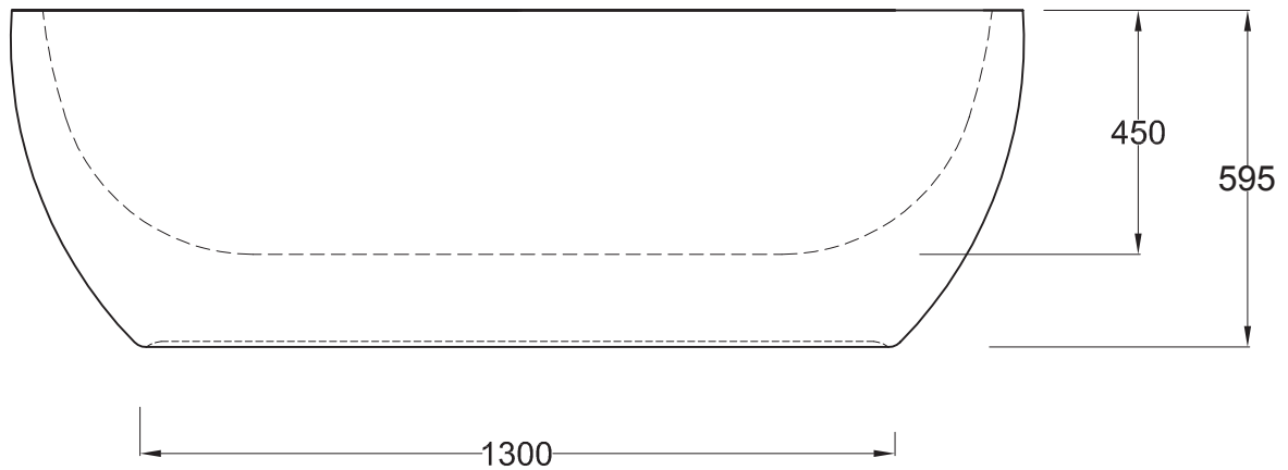
FRONT VIEW
